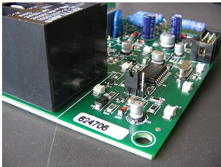
QuickTest jumper in position TEST
